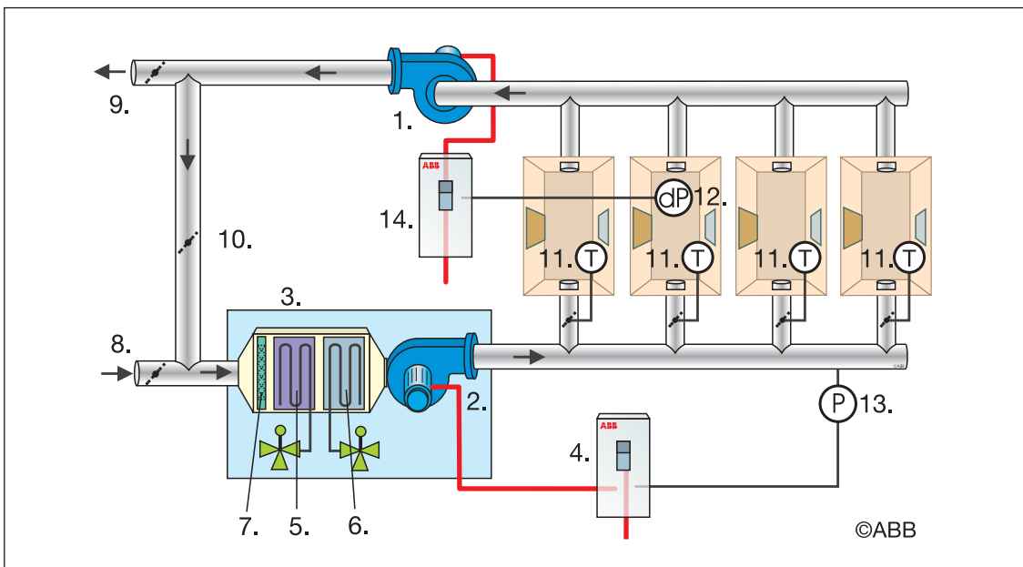
Variable air volume system with variable speed control fans.
