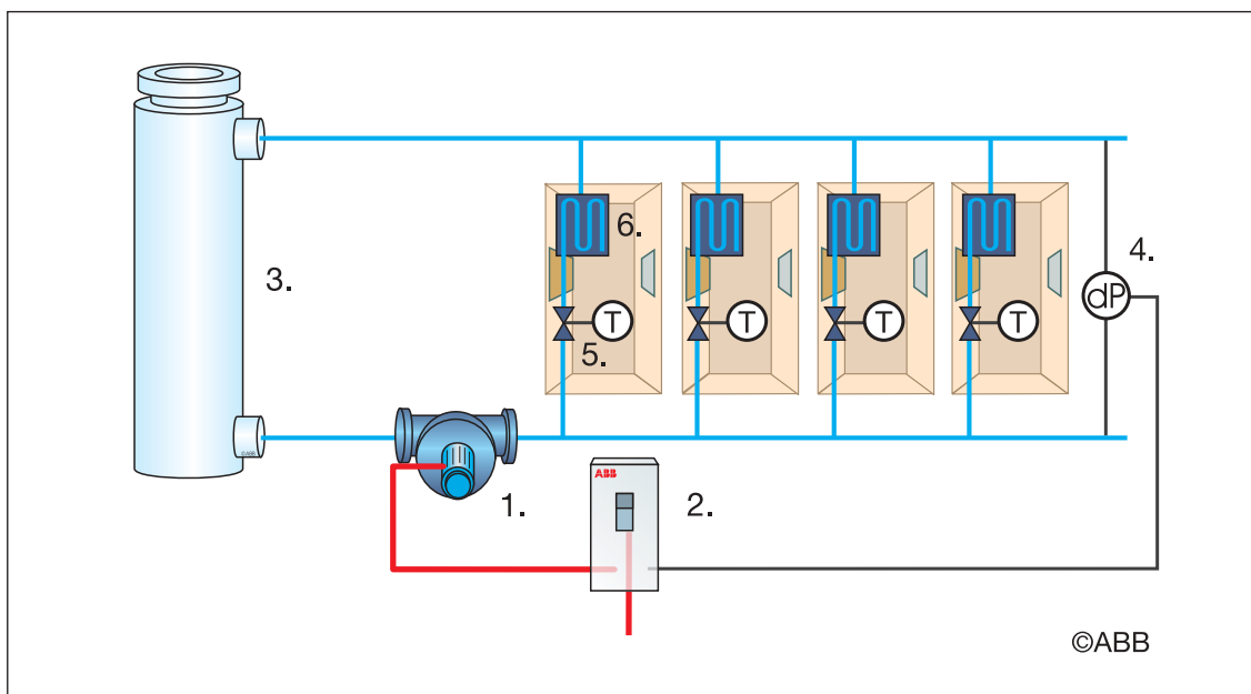
Chilled water system with variable speed drives.
