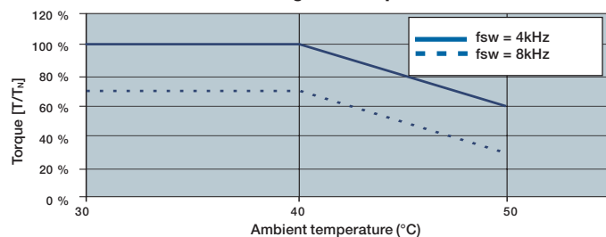
Derating with temperature
